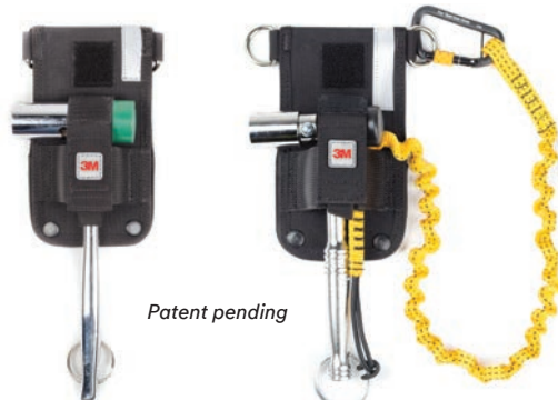
Back of holster features pouch for Safety Retractor (see page 124). Rear feed system allows retractor to tie off a scaffold wrench while staying out of the way.
